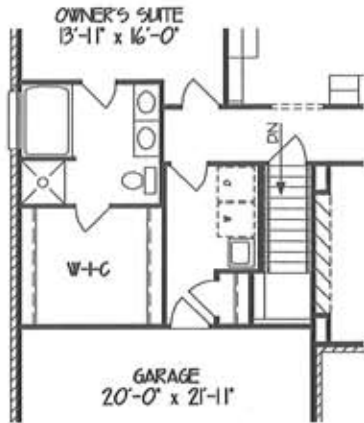
OPTIONAL LAYOUT W/ UPGRADED WALK-THROUGH LAUNDRY ROOM
