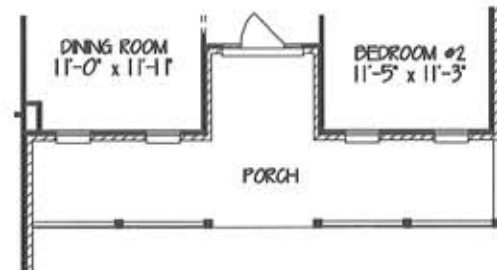
OPTIONAL FLOOR PLAN 'D' (INCL. FULL FRONT PORCH W/ DORMERS & FALSE GABLE. ADD 6" TO SIDE OF DINING RM) ADDS 3 SF
