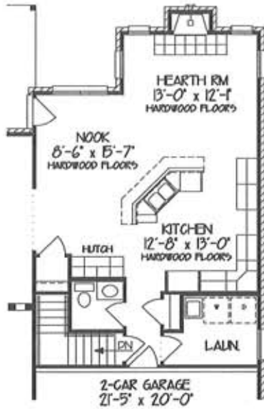
UPGRADED KITCHEN LAYOUT W/ OPTIONAL HUTCH
