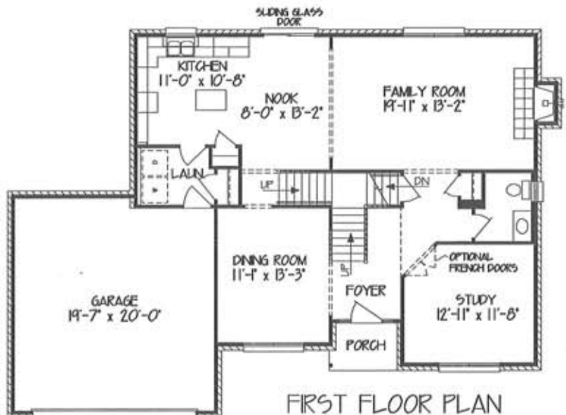
OPTIONAL STUDY & LAUN. RM LAYOUT WITH UPGRADED KITCHEN ADDS 192 SF
