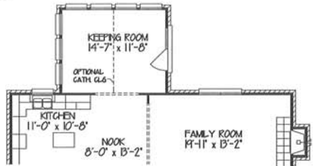
OPTIONAL KEEPING ROOM ADDS 192 SF
