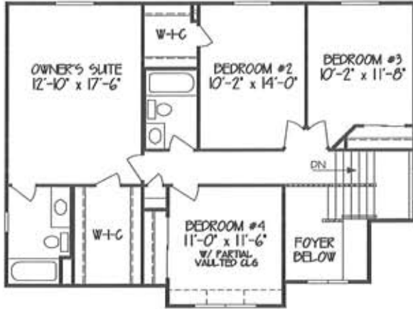
SECOND FLOOR PLAN 1113 SF
