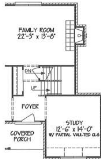
OPTIONAL FIRST FLOOR PLAN 'B' (INCL. STUDY, 2' ADDED TO FAM. RM SIDE OF HOME, & 2 SIDELIGHTS AT FRONT DOOR ADDS 294 SF
