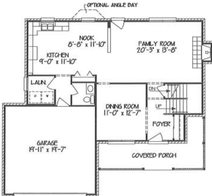
FIRST FLOOR PLAN 964 SF
