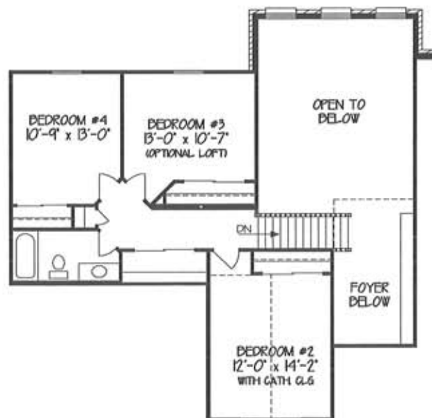
SECOND FLOOR PLAN 756 SF
