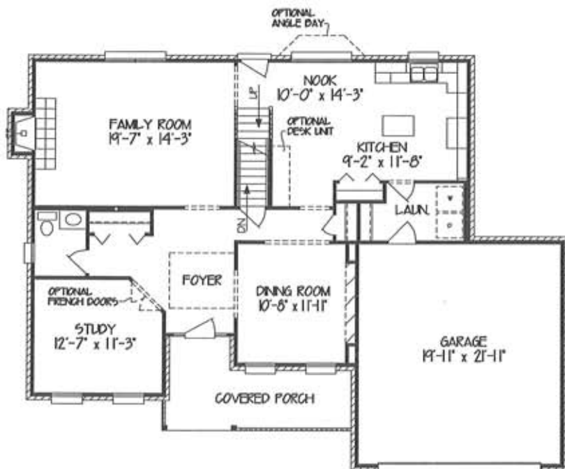
FIRST FLOOR PLAN 1261 SF
