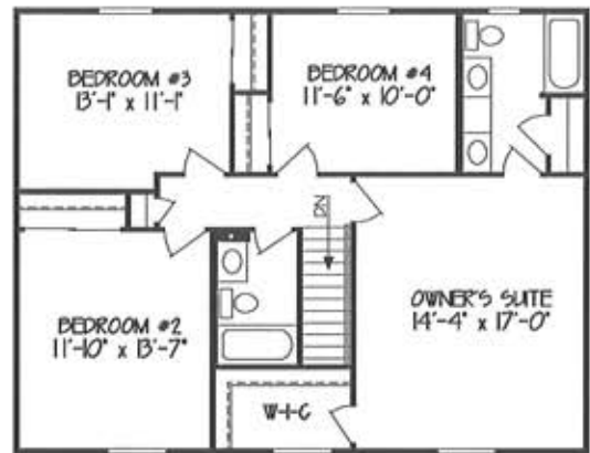
OPTIONAL 4-BDRM LAYOUT (ELEV. 'A') (INCL. 3 WINDOW FRONT & 2' TO 2ND FL REAR) ADDS 72 SF
