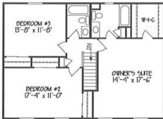
SECOND FLOOR PLAN 'A' 936 SF
