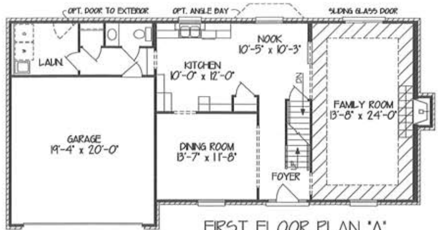
FIRST FLOOR PLAN 'A' 1074 SF
