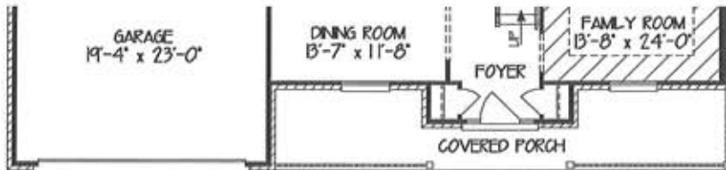
OPTIONAL FIRST & SECOND FLOOR PLANS 'B' (INCL. 4-BDRM LAYOUT, GABLE BUMP-OUT AT FRONT, LARGER GARAGE W/ FULL PORCH) ADDS 120 SF
