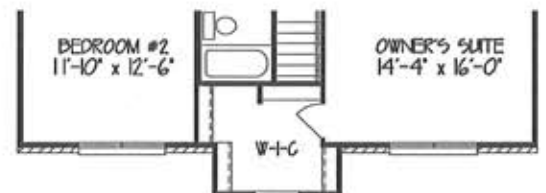
OPTIONAL FIRST & SECOND FLOOR PLANS 'C' (INCL. 4-BDRM LAYOUT, GABLE BUMP-OUT AT FRONT, & FRONT PORCH) ADDS 120 SF
