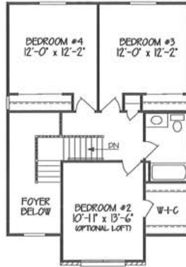
SECOND FLOOR PLAN 751 SF
